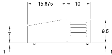
SIDE VIEW SCALE: 3/4"=1'-0"
